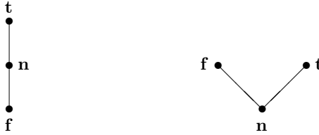
Figure 1: Hasse diagrams for the logical ordering of \{\mathbf{t}, \mathbf{f}, \mathbf{n}\} (left) and the approximation ordering of this set (right).
